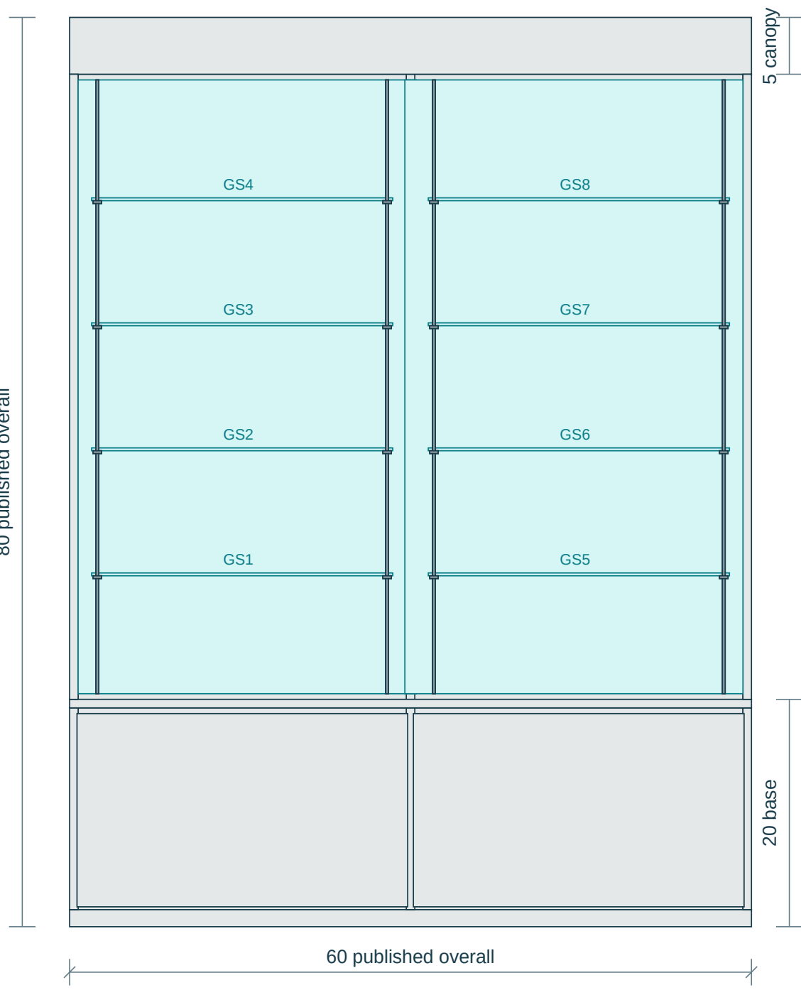
01 FRONT / FOUR ALIGNED LEVELS IN EACH BAY
